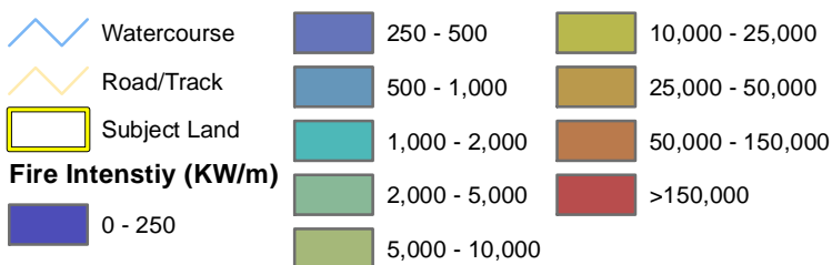
Figure 7: Bushfire Intensity
